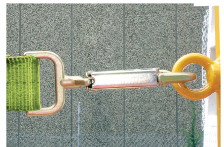
End post connection
