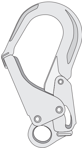
Double action scaffold hook - heavy duty
