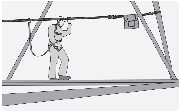
Example of a correctly rigged 3400UK
