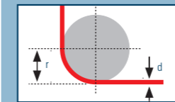
Definition of sharp edge: edge radius < thickness of sling gear.
