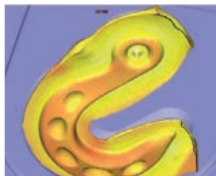
Material flow simulation
