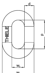
1) TWN 0089/1 Type SL = Short link
