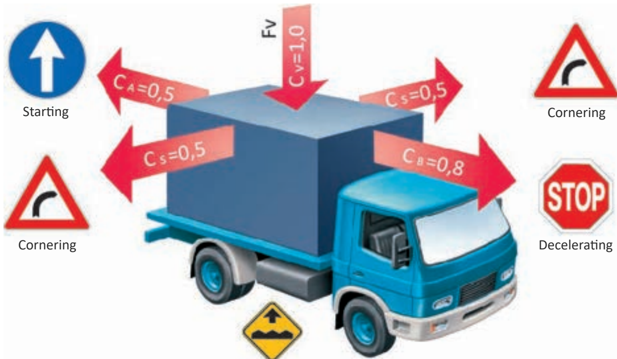
Vertical forces when driving
